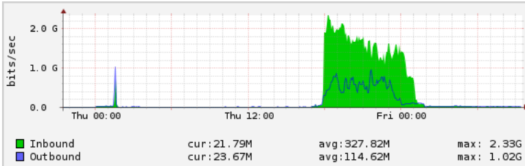
Device: prod-ent-ceph09.dc2.ec.loc Component: bond0.300 Graph: Throughput
